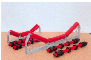
Supports
